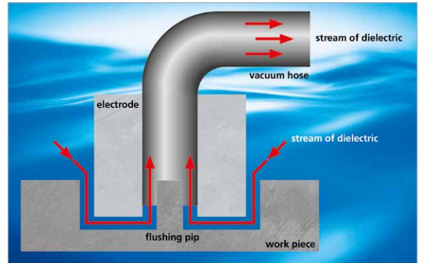
Figure 4: Suction flushing
