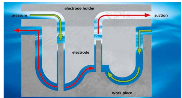
Figure 5: Combined flushing
